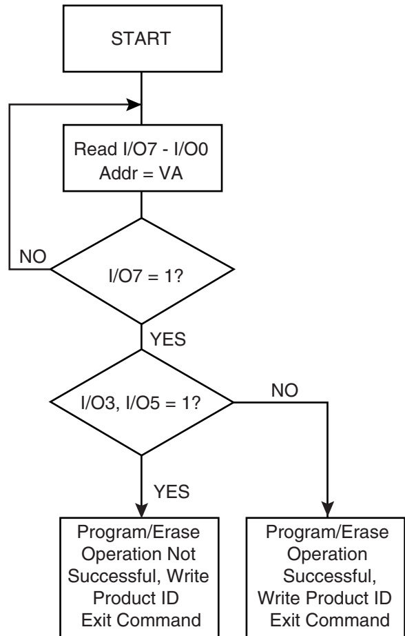
Figure 3-3. Data Polling Algorithm (Configuration Register = 01)
